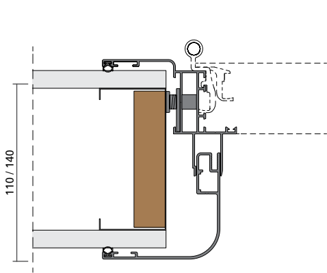
IMBOTTE 2 - spessore 110/140 mm / JAMB 2 - thickness 110/140 mm
